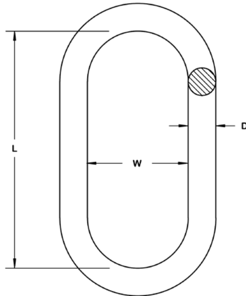
FIGURE 33. Type XV, end link.
