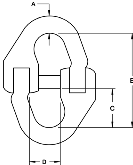
FIGURE 32. Type XIV, mechanical coupling link.
