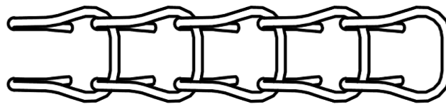
FIGURE 12. Type II, class 9, weldless ladder chain.
