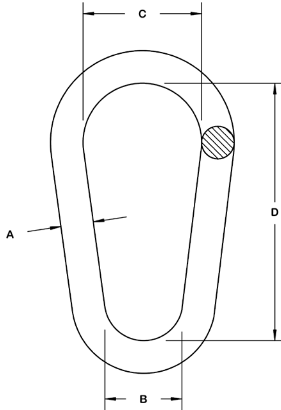
FIGURE 31. Type XIII, pear-shaped link.
