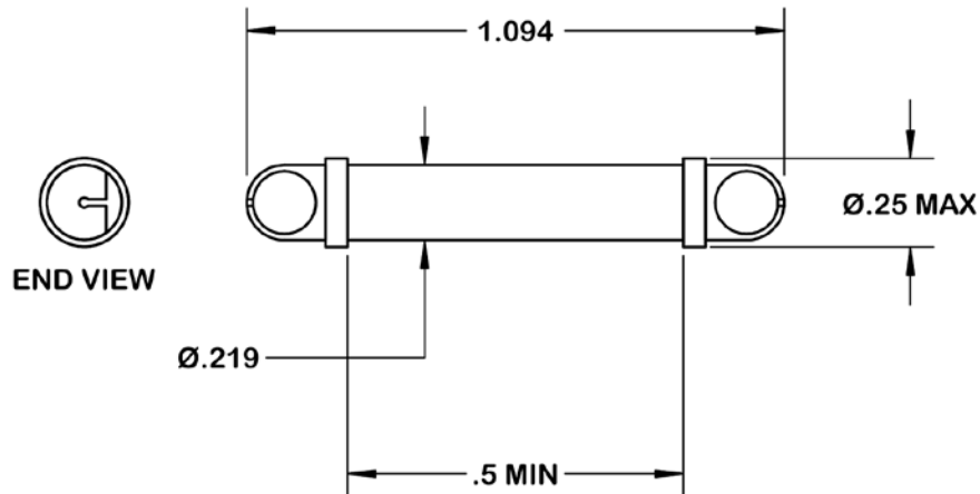
FIGURE 30. Type XI, bead-chain insulating coupling .
